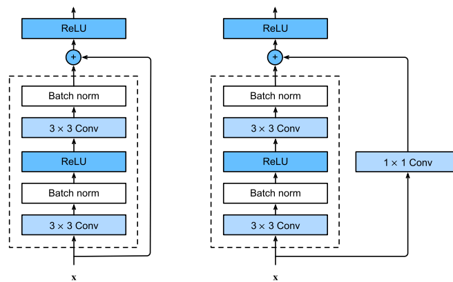
Fig. 8.6.3 ResNet block with and without 1 \times 1 convolution, which transforms the input into the desired shape for the addition operation.
