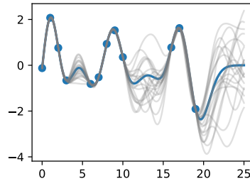
Fig. 18.1.4 Posterior samples, alongside posterior mean, which can be used for point predictions, in blue.
