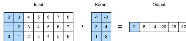
Fig. 16.3.4 Two-dimensional cross-correlation operation with a single input channel. The shaded portions are the first output element as well as the input and kernel tensor elements used for the output computation: 2 \times (-1) + 3 \times (-3) + 1 \times 3 + 2 \times 4 + 0 \times 1 + 1 \times 2 = 2 .
