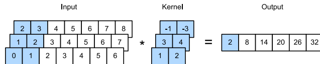
Fig. 16.3.3 One-dimensional cross-correlation operation with 3 input channels. The shaded portions are the first output element as well as the input and kernel tensor elements used for the output computation: 0 \times 1 + 1 \times 2 + 1 \times 3 + 2 \times 4 + 2 \times (-1) + 3 \times (-3) = 2 .
