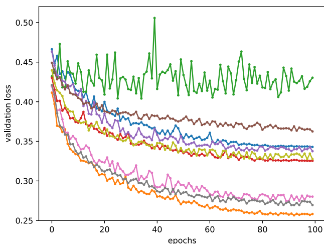
Fig. 19.4.1 Learning curves of random hyperparameter configurations
