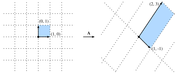
Fig. A.9 The matrix \mathbf{A} again distorting the grid. This time, I want to draw particular attention to what happens to the highlighted square.
