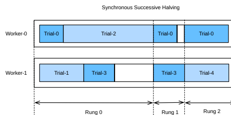
Fig. 19.5.1 Synchronous successive halving with two workers.
