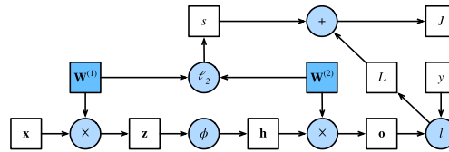
Fig. 5.3.1 Computational graph of forward propagation.
