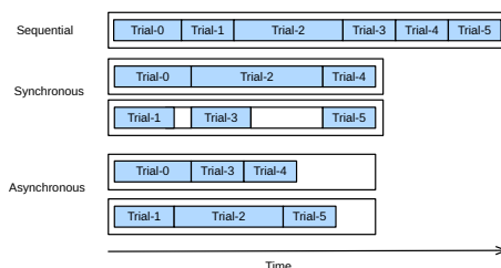
Fig. 19.3.1 Distributing the hyperparameter optimization process either synchronously or asynchronously. Compared to the sequential setting, we can reduce the overall wall-clock time while keep the total compute constant. Synchronous scheduling might lead to idling workers in the case of stragglers.
