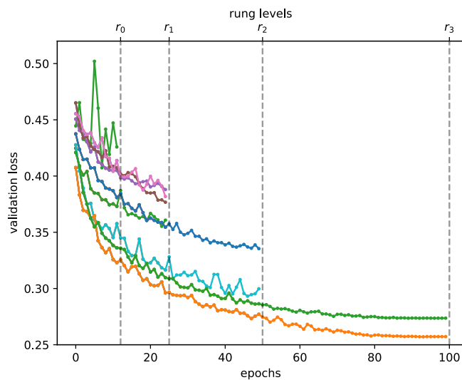
Fig. 19.4.2 Learning curves of random hyperparameter configurations.
