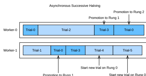
Fig. 19.5.2 Asynchronous successive halving (ASHA) with two workers.
