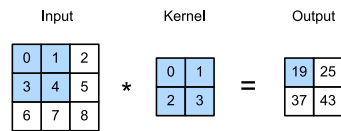
Fig. 7.2.1 Two-dimensional cross-correlation operation. The shaded portions are the first output element as well as the input and kernel tensor elements used for the output computation: 0 \times 0 + 1 \times 1 + 3 \times 2 + 4 \times 3 = 19 .
