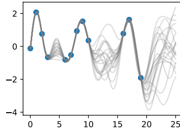
Fig. 18.1.3 Sample posterior functions, once we have observed the data.
