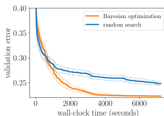
Fig. 19.2.1 Example any-time performance plot to compare two algorithms A and B.
