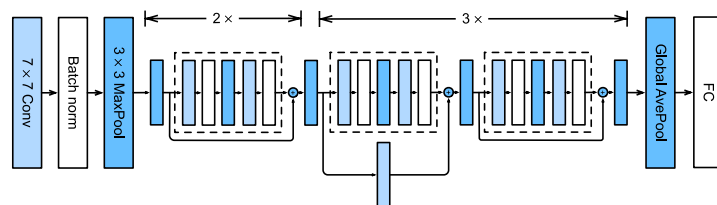
Fig. 8.6.4 The ResNet-18 architecture.
