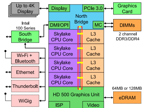
Fig. 13.4.3 Intel Skylake consumer quad-core CPU.
